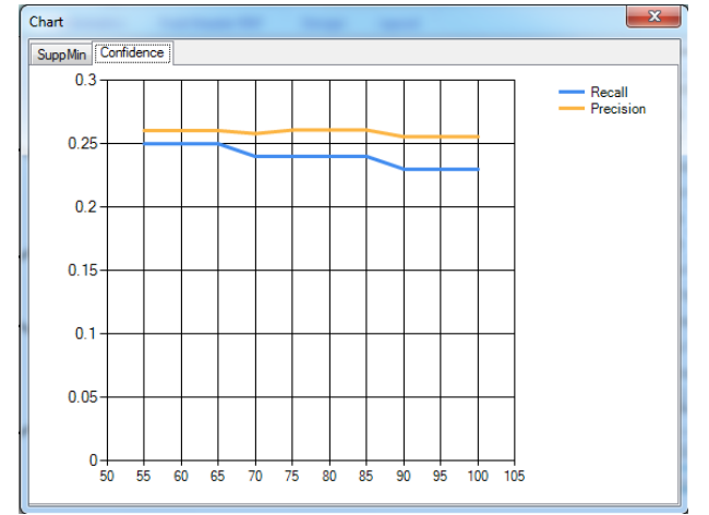
3b. conf_{min}
