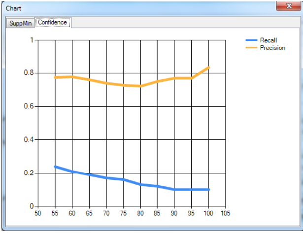
2b. conf_{min}
